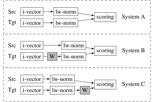
Figure 2: Three proposed approaches for the comparison of i -vectors. In systems B and C, a projection matrix W trained from different languages is used for comparing i -vectors.
