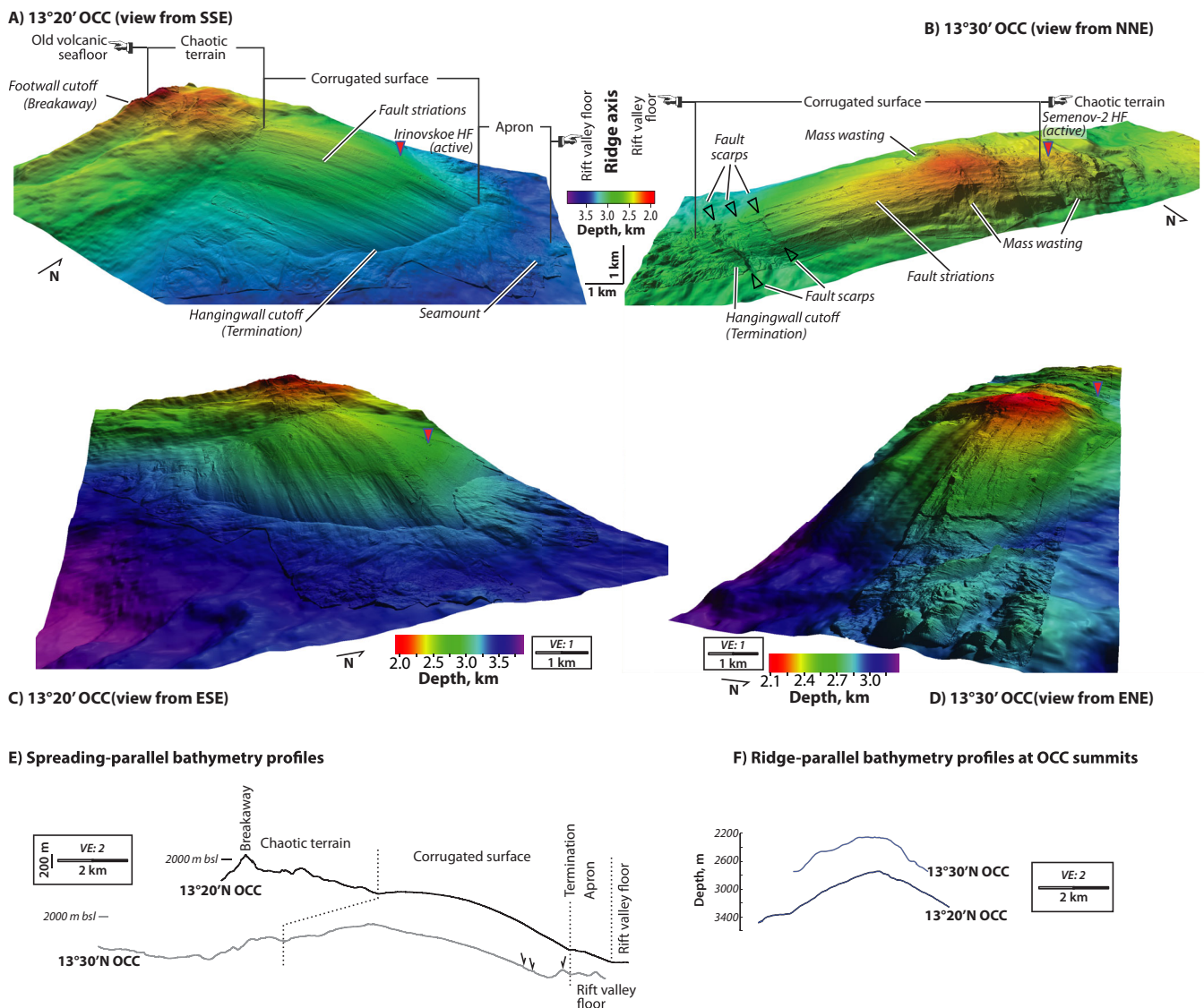
Figure 3. Three-dimensional views of (A) the 13°20'N OCC microbathymetry (Figures 2C and 2D), viewed from the SSE, and (B) the 13°30'N OCC (Figures 2A and 2B) viewed from the NNE, showing the different structural domains together with other morphologic features (all discussed in the text). Additional views from the ridge axis of both the (C) 13°20'N OCC and the (D) 13°30'N OCC are also shown. Active hydrothermal fields (HF) are indicated in the four panels (upside-down triangles, filled red). (E) Bathymetric profiles parallel to the spreading direction along the center of both detachments. Location and limits of the different terrains identified are shown. The profiles have been aligned at their terminations, and vertically offset for clarity. The 2000 m depth is indicated as a horizontal bar for each profile. (F) Bathymetric profiles parallel to the ridge axis and across the summit of both OCCs' corrugated surface . The along-axis profiles are shown with no offset in depth. Profiles in both Figures 3E and 3F are shown with a vertical exaggeration (VE) of 2.
