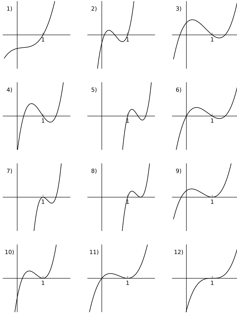
Figure 1: All possible roots of a cubic r.h.s. of (16):
