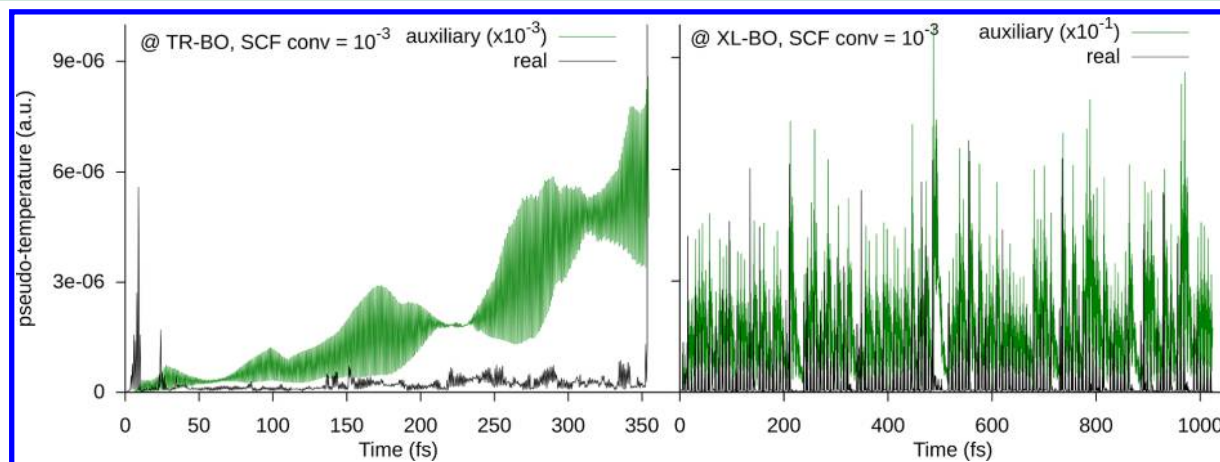
Figure 4. Comparison between the QM/AMOEBA auxiliary and real EDF pseudotemperature for SCF convergence set to 10^{-3} in arbitrary units (au). The values for the auxiliary EDFs are scaled by a factor 10^{-3} for TR-BO and 10^{-1} for XL-BO to obtain comparable scales.
