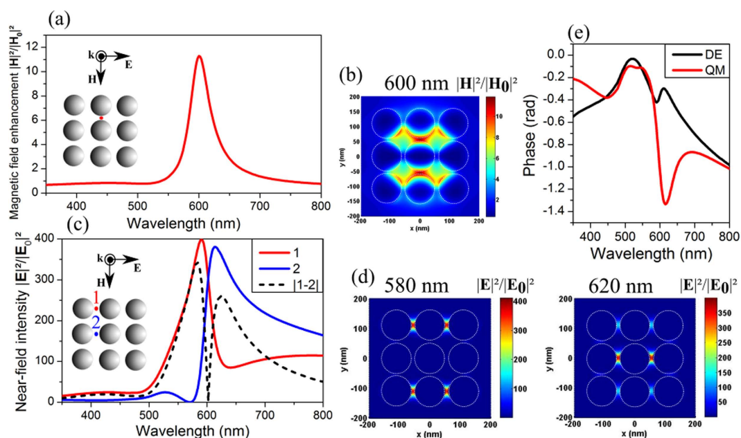
Figure 5. (a) Magnetic field enhancement in the structure with (b) the magnetic field mapping at 600 nm. (c) Near-field intensities and contrast between the two first lines of the array versus wavelength with (d) near-field mapping at 580 nm and 620 nm. (e) Phase of the complex extinction of dipolar electric and quadrupolar magnetic multipoles. All the near-fields and phases are calculated using the analytical Mie theory.
