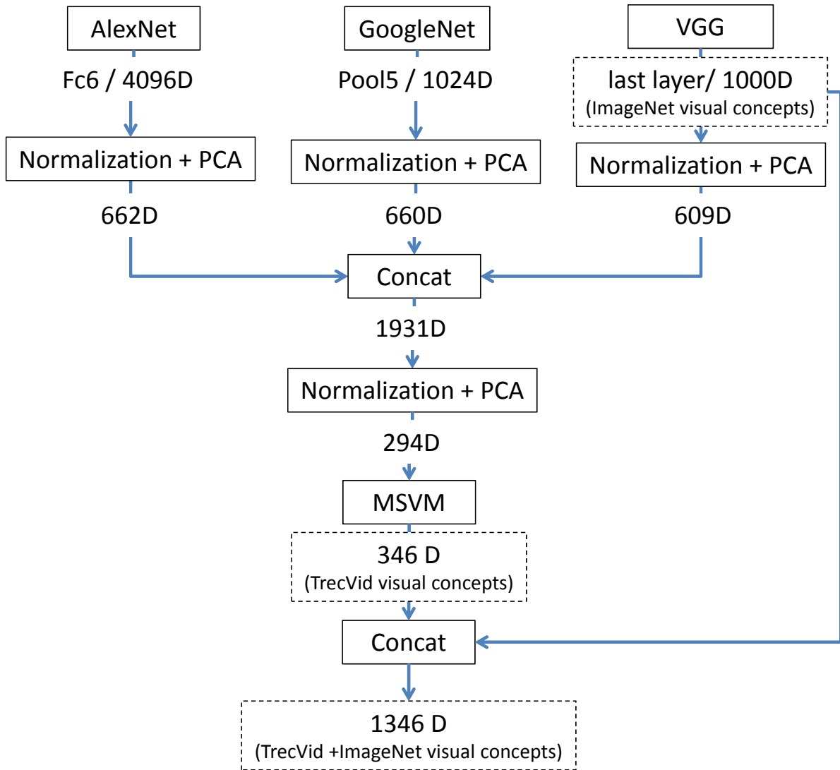
Figure 1: MRIM Lifelog Visual indexing
