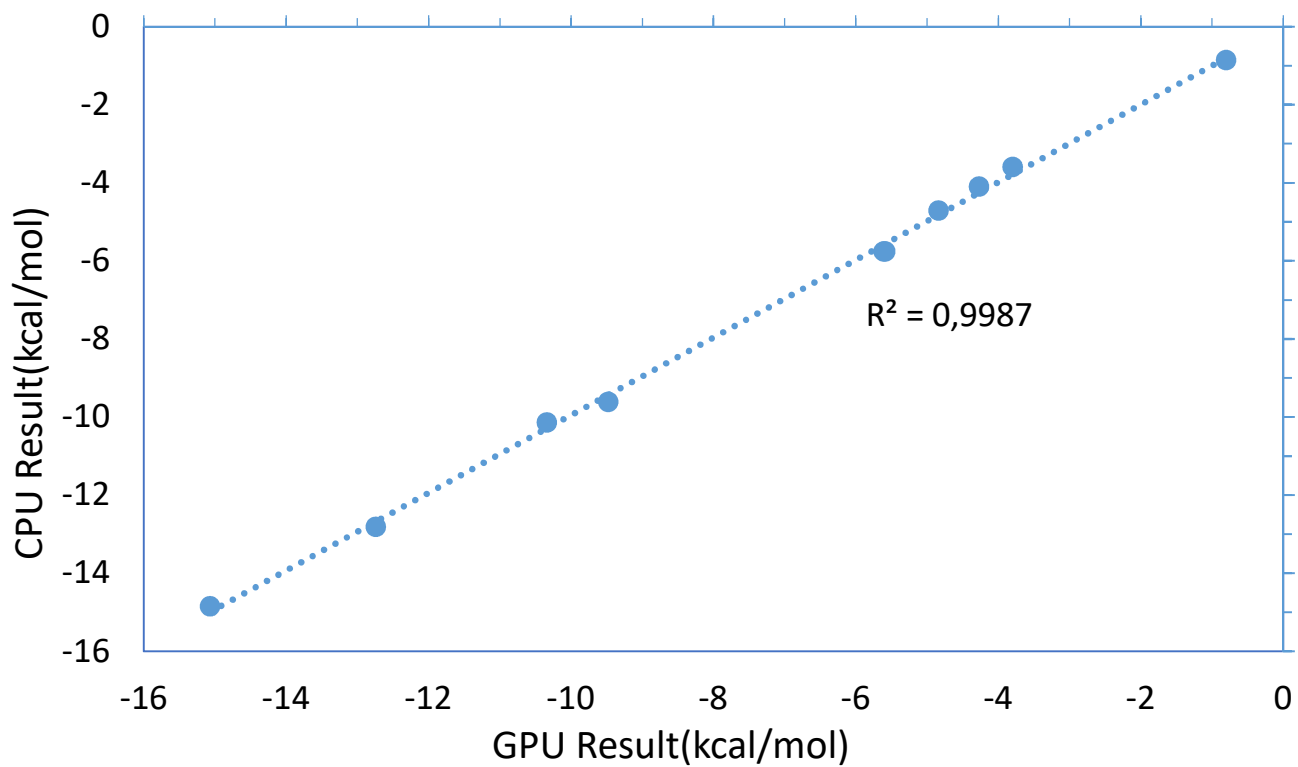
Figure 6: Comparison between the calculated solvation free energies for the 10 molecule aromatic compound dataset on the Tinker-OpenMM GPU and Tinker CPU platforms.
