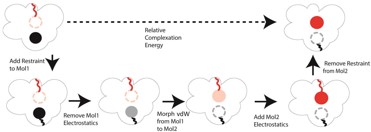
Figure 2: Path used to determine the relative complexation interaction energy of two ligands using a dual topological approach.
