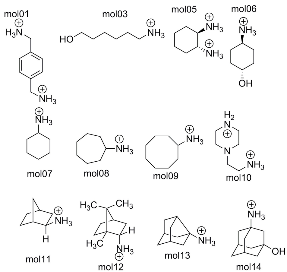
Figure 3: Structures of the 12 sampl4 molecules utilized in this study.
