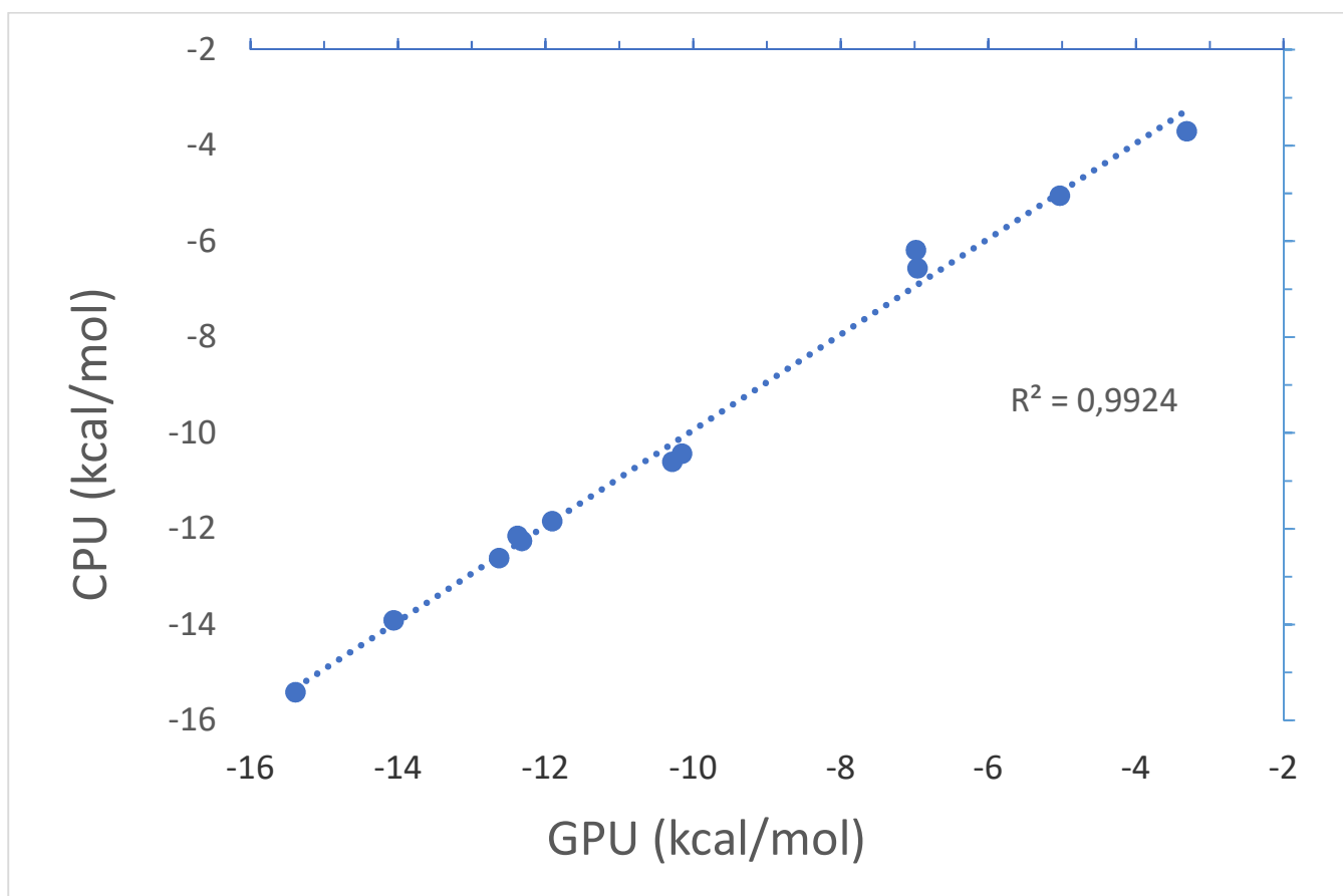
Figure 5: Comparison between the sampl4 binding free energies of 12 sampl4 compounds computed by the Tinker-OpenMM GPU and Tinker CPU platforms. GPU simulations were run for 5ns at each perturbation step, while CPU simulations were run for 1ns.
