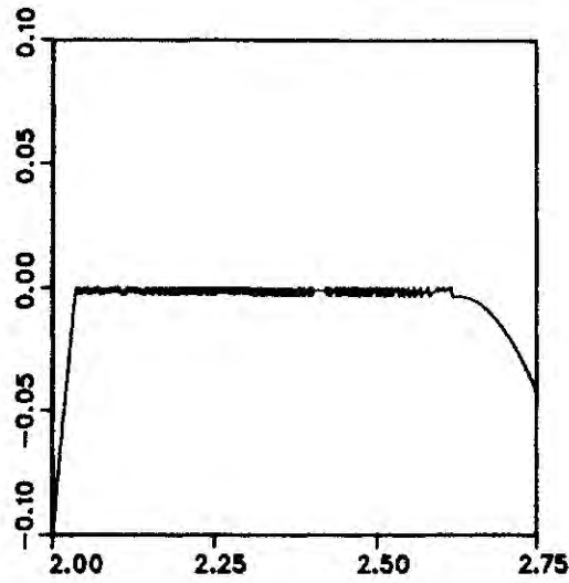
FIG. 6. Approximation of z(\cdot) by Runge-Kutta method with h = 0.001 .
