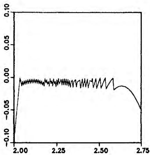
FIG. 4. Approximation of z(\cdot) by Runge-Kutta method with h = 0.005 .
