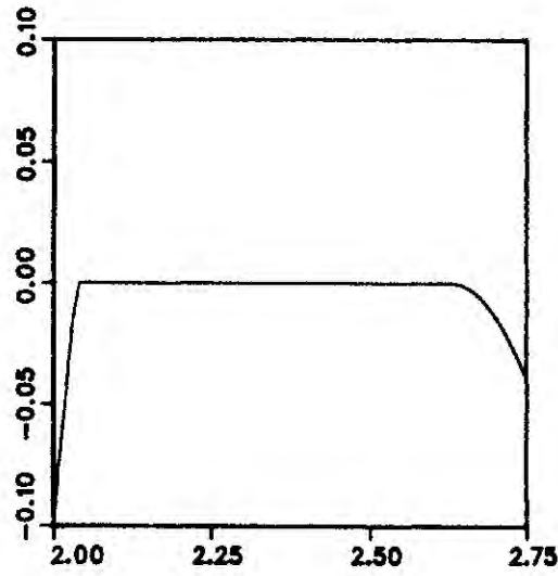
FIG. 5. Approximation of z(\cdot) by implicit midpoint rule with h = 0.005 .
