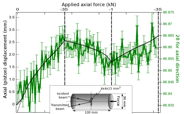
Fig. 1 Macroscopic axial displacement (initial loading cycle in grey) and change in 2\theta for grain-strain in the axial direction (average over the gauge volume see in-set) as functions of the applied axial force. Inset - measurement and loading set-up.
