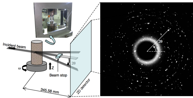
Fig. 2 3DXRD set-up and (to right) example diffraction pattern from a single \omega angle for the 10 mm oedometer.
