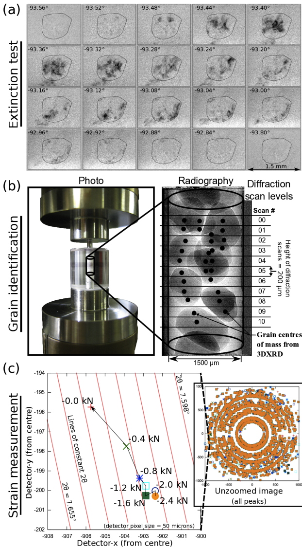
Fig. 3 (a) Extinction test: radiographs after subtraction of the average of the first and last in sequence (to remove approximately direct beam image) at 0.04^\circ steps from -93.56^\circ to -92.80^\circ . (b) Comparison of centres-of-mass from 3DXRD and grain positions from radiography (1.5 mm oedometer), (c) Movement of a selected Bragg peak, for a grain at the centre of the 10 mm oedometer sample, as a function of decreasing load.
