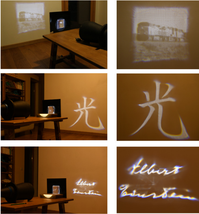
Figure 16: Fabricated lenses for a collimated light source. From left to right: experimental setup, zoom on the target screen. From top to bottom: TRAIN, HIKARI, EINSTEIN'S SIGNATURE targets. Images are focused on a screen at 2 meters for the first two rows and 1 meter for the last one.
