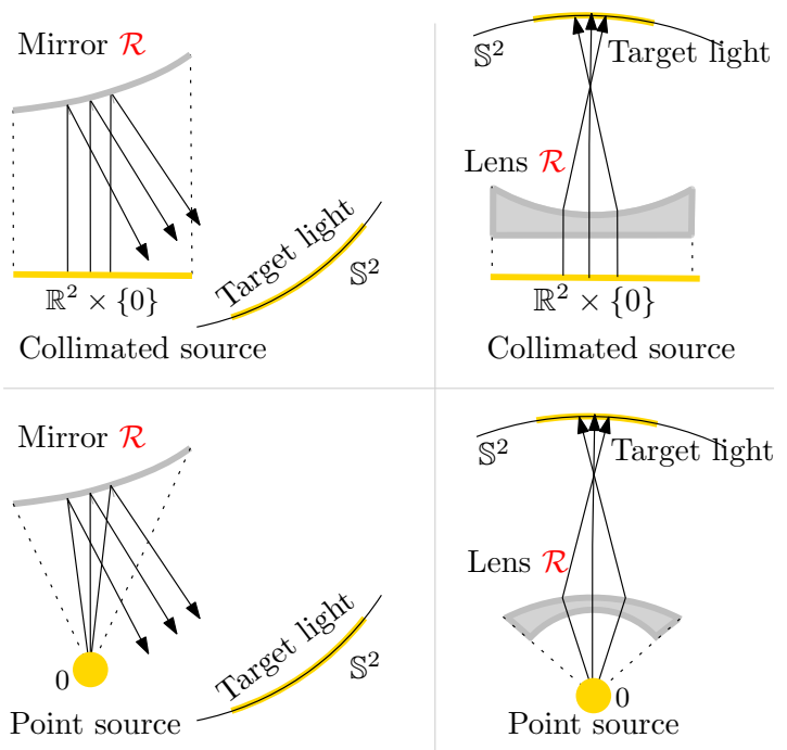
Figure 2: Four inverse problems arising in non-imaging optics. In each case, the goal is to build the surface \mathcal{R} of a mirror or a lens. For each problem, we provide two solutions (for instance, convex or concave surfaces when the light source is collimated). Top/Bottom: Collimated light sources/Point light sources. Left/Right: Mirror/Lens design.
