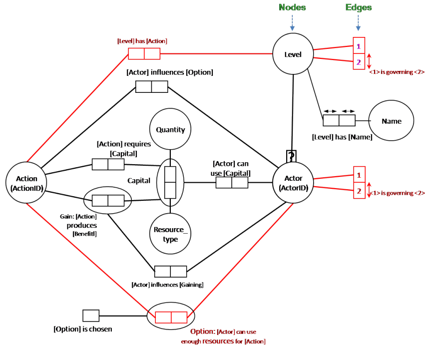
Figure 4 – The AiC Metamodel
