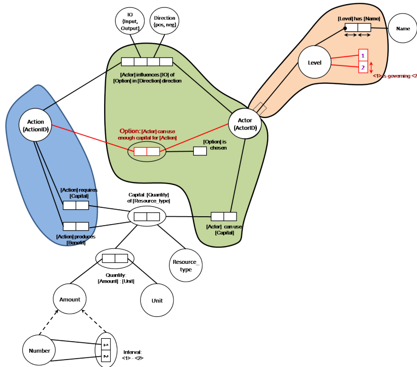
Figure 10 – Grouping the AiC Metamodel
