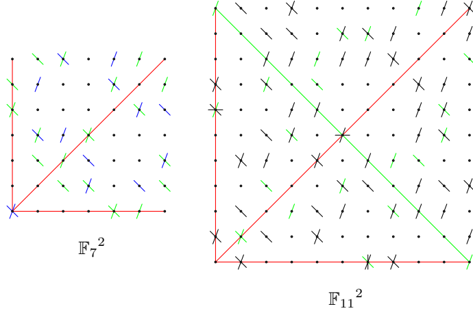
Figure 3: Lines of the minimal Besicovitch arrangement in \mathbb{F}_d^2 providing the complexity C_d where d = 7 (on the left) and d = 11 (on the right). Red lines are those of \{L_0, L_{-1}, L_\infty\} , green ones are those of \{L_1, L_{\frac{d-1}{2}}, L_{-2}\} , blue ones are those of \{L_\omega, L_{\omega^2}\} and black ones are lines of a 6-cycle. The number of all but the simple points is 25 for d = 7 , and 67 for d = 11 ; thus C_7 = 25 and C_{11} = 67 .
