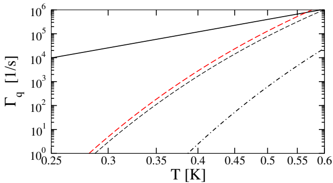
FIG. 1: Phonon damping rates at angular frequency \omega_{\mathbf{q}} = 2\pi \times 165 GHz ( q = 0.3\text{\AA}^{-1} ) in liquid {}^4\text{He} at pressure P = 20 bar as functions of temperature. Solid line: purely phononic damping \Gamma_{\phi\phi} due to Landau-Khalatnikov four-phonon processes [1, 6, 16]; it depends on the curvature parameter \gamma defined as \omega_{\mathbf{q}} = cq[1 + \frac{\gamma}{8}(\frac{\hbar q}{mc})^2 + O(q^4)] . Interpolating measurements of P \mapsto \gamma(P) in Refs.[20, 21] gives \gamma = -6.9 . Dashed black line/dash-dotted black line: damping due to scattering/absorption-emission by rotons, see Eq.(12)/(15). Red dashed line: original formula of Ref.[1] for the damping rate due to phonon-roton scattering. The roton parameters are extracted from their dispersion relation k \mapsto \epsilon_{\mathbf{k}} measured at various pressures [22]: \Delta/k_B = 7.44\text{K} , k_0 = 2.05\text{\AA}^{-1} , m_*/m = 0.11 , \rho k'_0/k_0 = 0.39 , \rho\Delta'/\Delta = -1.64 , \rho^2\Delta''/\Delta = -8.03 , \rho m'_*/m_* = -4.7 . In Eq.(15), parabolic approximation (9) is used (hence \epsilon_{k_*}/\Delta \simeq 1.43 ). The speed of sound c = 346.6 m/s, and the Grüneisen parameter \frac{d \ln c}{d \ln \rho} = 2.274 entering in \Gamma_{\phi\phi} , are taken from equation of state (A1) of Ref.[23]. The low values \frac{\hbar q}{mc} = 0.13 and \frac{k_B T}{mc^2} < 10^{-2} justify our use of quantum hydrodynamics.
