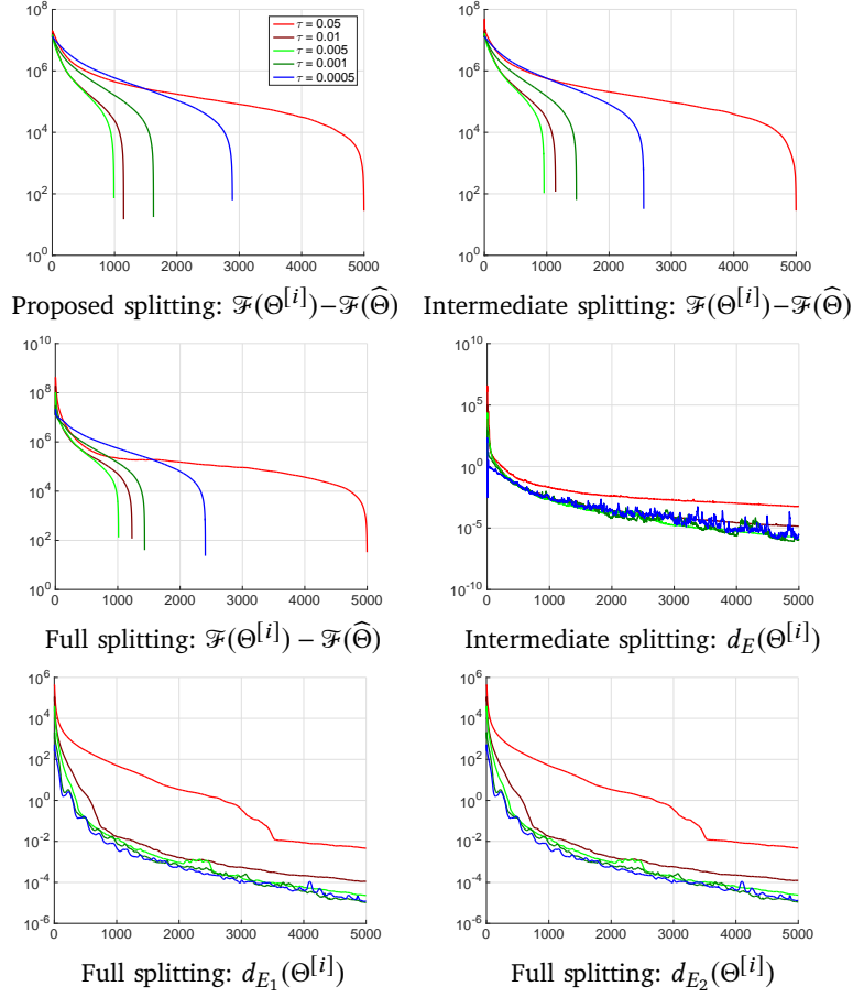
Fig. 2. Evolution of different criteria with respect to the iteration number, for different values of the parameter \tau . d denotes the distance to a convex set. d_E is zero for the proposed method.
