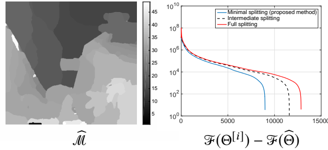
Fig. 3. Estimated disparity map (right) and convergence behavior with respect to computation time for \tau = 0.005 .
