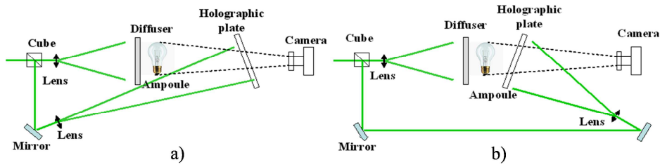
Figure 28. Image transmission holography (a) and image reflection holography (b)
