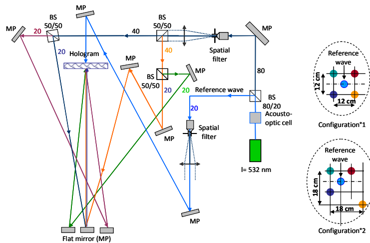
Figure 15. Optical setup defined for recording of reflection holographic grating
