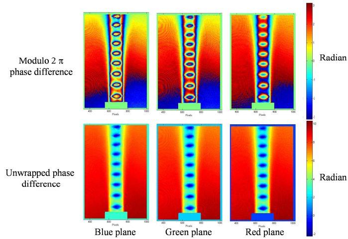
Figure 6. Maps of RGB phase difference (modulo 2\pi and unwrapped) – P = 3 bars
