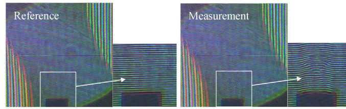
Figure 11. Interference micro-fringes recorded for the reference and the measurement – P = 4 bars
