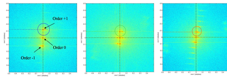
Figure 12. 2D spectra computed on the three channels for the reference interferogram - P= 4 bars
