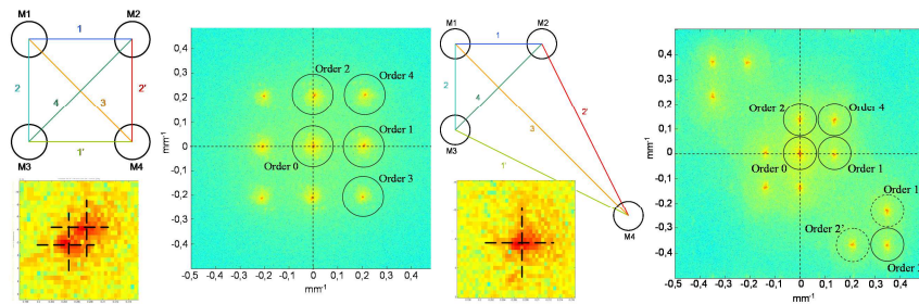
Figure 17. Position of four mirrors (square and kite) at the recording, localization of different diffraction orders in 2DFFT plane and zoom of +1 order.
