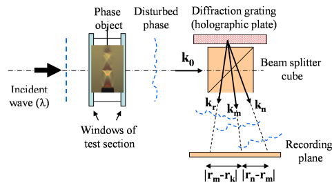
Figure 14. Principle of self-referenced digital holography by reflection
