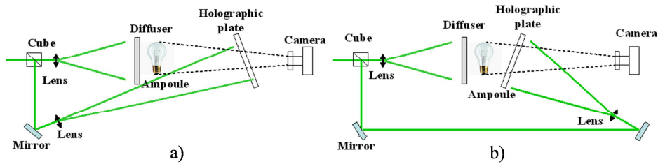
Figure 28. Image transmission holography (a) and image reflection holography (b)
