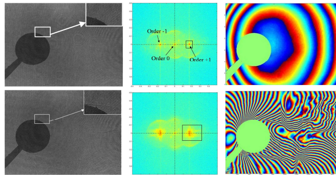
Figure 24. Interferograms analysis at Mach 0.73
