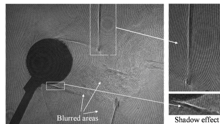
Figure 20. Highlighting of blurred areas and shadow effect – Mach 0.73
