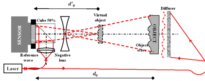
Figure 26. Stochastic digital holographic setup
