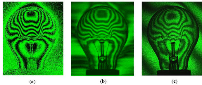
Figure 29. Comparison between intensity of fringes, (a) fringes calculated with digital holography, (b) fringes obtained with transmission holography, (c) fringes obtained with reflection holography
