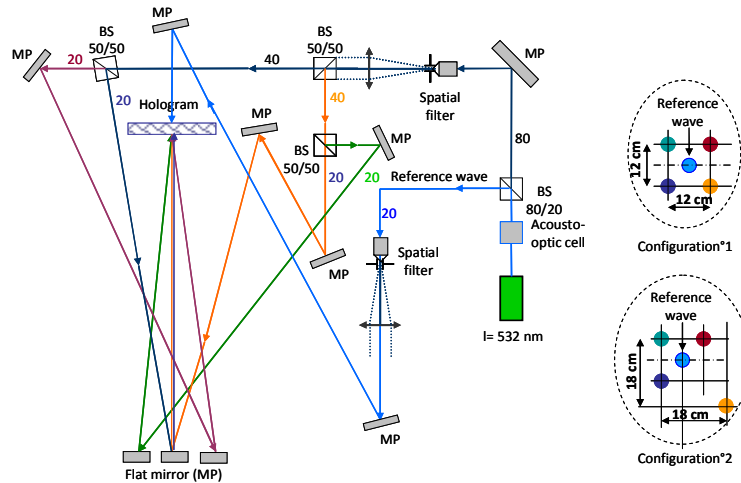
Figure 15. Optical setup defined for recording of reflection holographic grating
