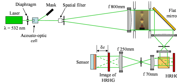
Figure 16. Digital holographic interferometer without reference
