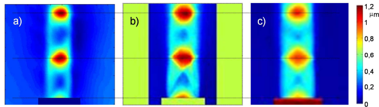
Figure 19. Comparison of experimental results obtained for three different interferometric techniques for a pressure at P=5 bars, (a) Without reference setup, (b) Michelson set-up, (c) Wollaston setup.
