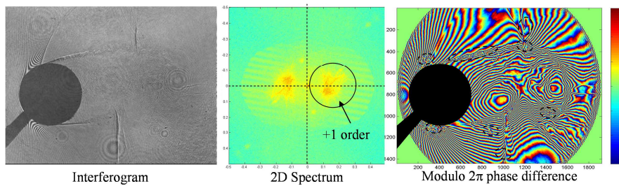
Figure 22. Interferogram analysis at Mach 0.73 – Residual phase shifts
