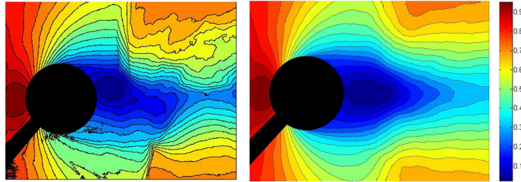
Figure 25. Instantaneous and averaged gas density fields ( \rho/\rho_0 ) – Mach 0.73
