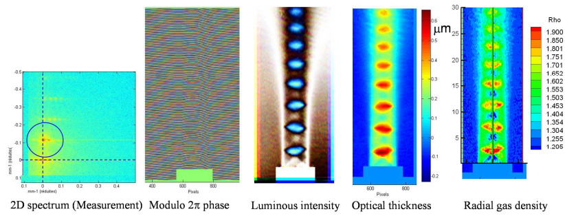
Figure 13. Analysis of the case for red channel P = 3 bars (from spectrum to gas density)
