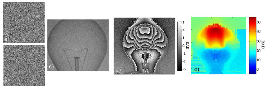
Figure 27. Quantitative measurement inside the bulb, a) virtual phase extracted from numerical reconstruction (bulb off), b) bulb lighting, c) image amplitude of the strand, d) modulo 2\pi phase computed from (a) and (b), e) unwrapping of (d)
