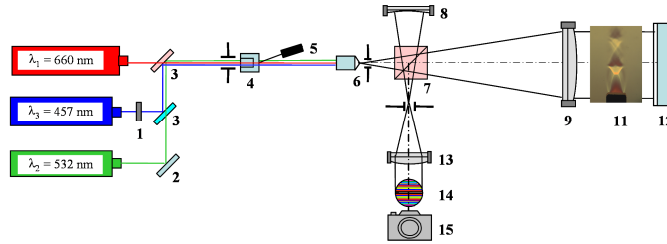
Figure 3. Michelson digital holographic interferometer
