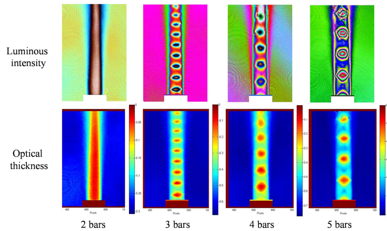
Figure 7. Evolution of the luminous intensity and the optical thickness with the pressure
