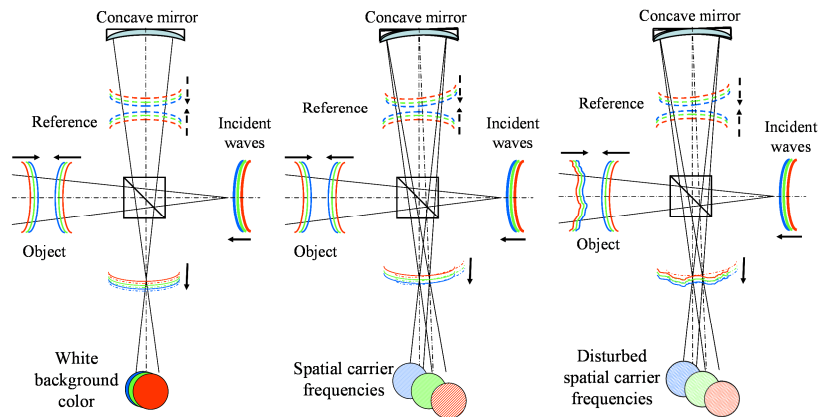
Figure 4. Generation and micro-fringes formation by the transparent object
