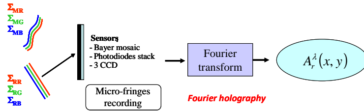
Figure 2. Fourier holography for measuring transparent objects
