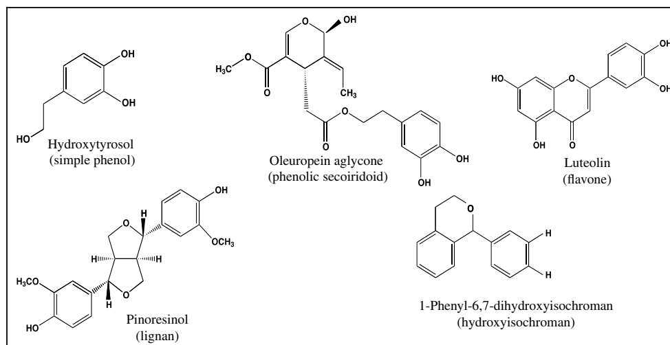
Fig. 1. Phenolic structures of olive oil and their sub-categories (in brackets).
