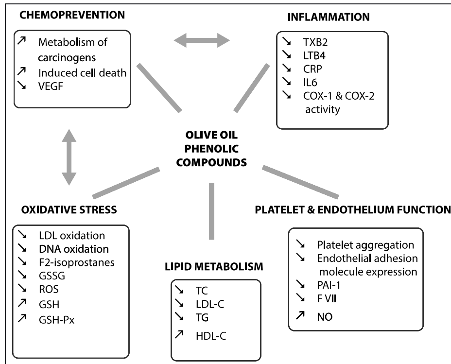
Fig. 2. Different actions of olive oil phenolic compounds.
