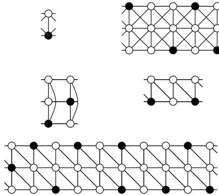
Figure 5: Periodic patterns for minimum density LD-codes of infinite king, triangular and toroidal strips of heights 2, 3.
