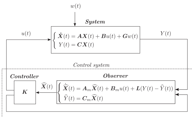
FIG. 3. Diagram of the control system.
