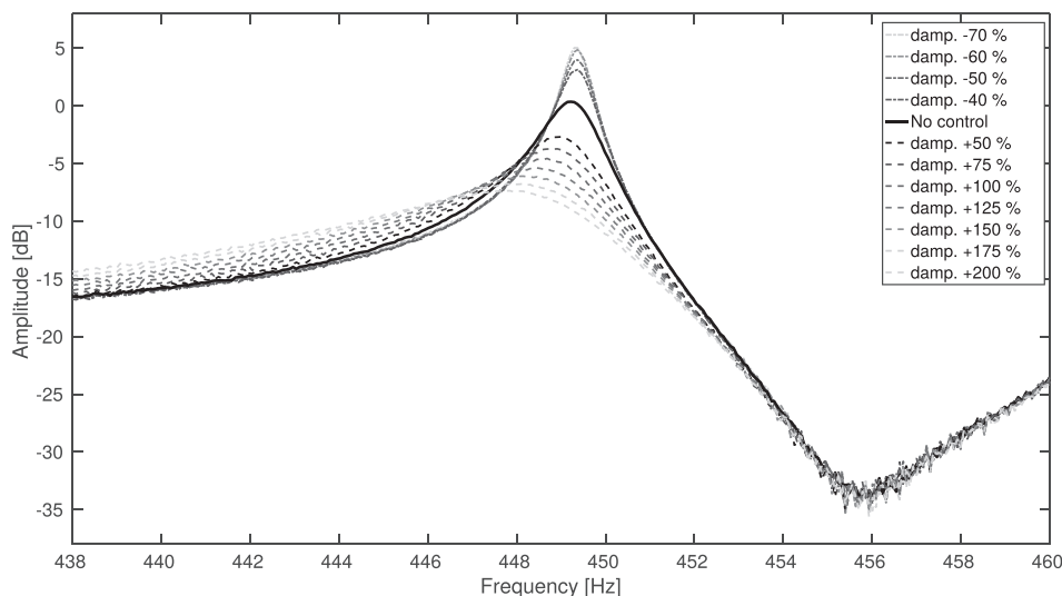
FIG. 8. Experimental sensor-actuator FRF without control and for various damping control factors.
