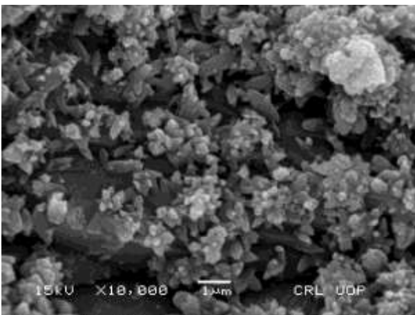
Figure. 20 SEM of sample M2, X10000 at 1 \mu\text{m}
