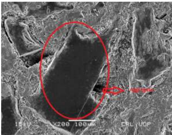
Figure. 15 SEM of sample M2, X200 at 100 μm
