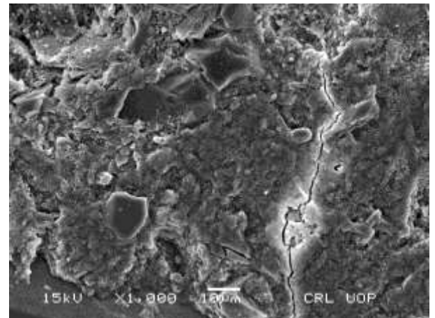
Figure. 24 SEM of sample M3, X1000 at 10 \mu\text{m}
