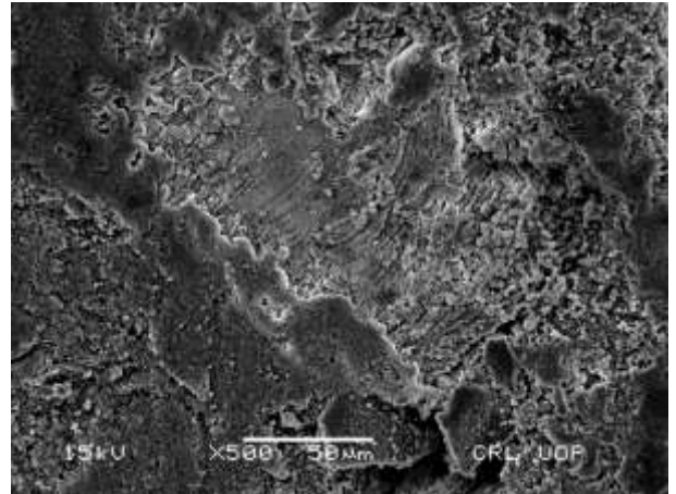
Figure. 16 SEM of sample M2, X500 at 50 μm
