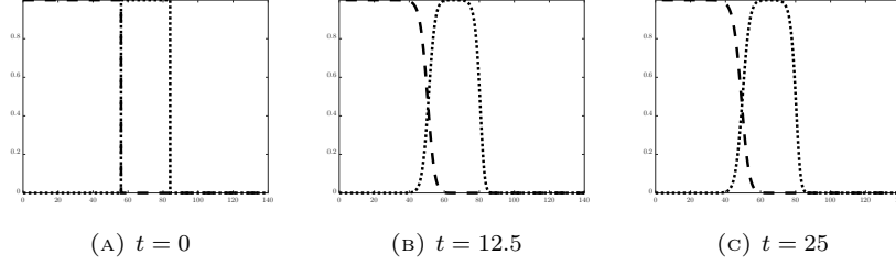
FIGURE 1.1. Numerical simulation of the convergence to a non-monotonic competition–diffusion monostable traveling wave with minimal speed ( u_1 dashed line, u_2 dotted line, x - 2t as horizontal axis).
