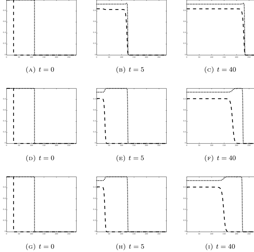
FIGURE 1.3. Numerical simulations of the monostable case with initial data corresponding to a competition–diffusion terrace ( u_1 dashed line, u_2 dotted line, x as horizontal axis).
