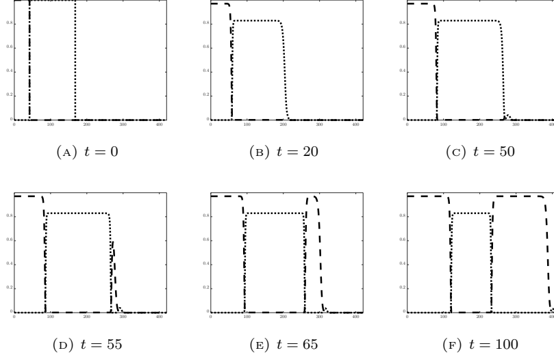
FIGURE 1.2. Numerical simulation of the bistable case with initial data corresponding to a competition–diffusion terrace ( u_1 dashed line, u_2 dotted line, x as horizontal axis).
