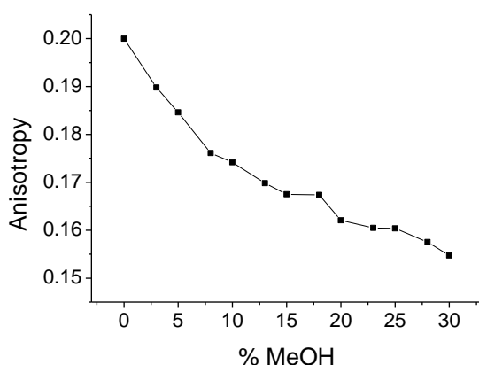
Figure 5: Fluorescence anisotropy of RhB-labeled Mb in water/MeOH mixture.
