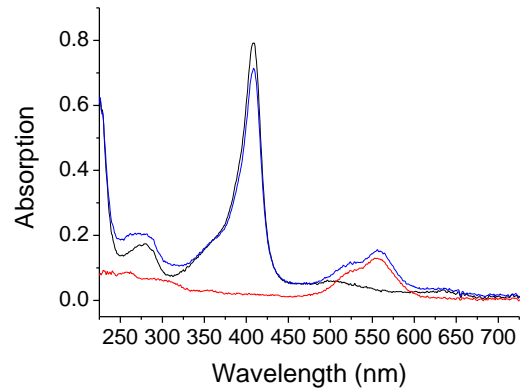
Figure 3: Absorption spectra of (black) Mb, (red) RhB and (blue) RhB-labeled Mb in 10 mM PBS buffer.
