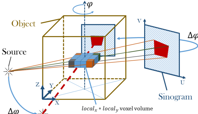
Fig. 1. 3D Computed Tomography Projection.
