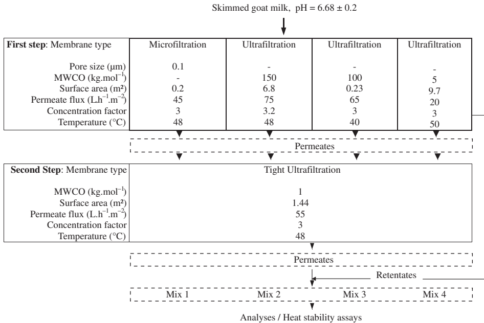
Figure 1. Schematic outline of the membrane process used to reduce the whey protein content of goat milk. Reconstitution of modified milk was performed at constant casein concentration.
