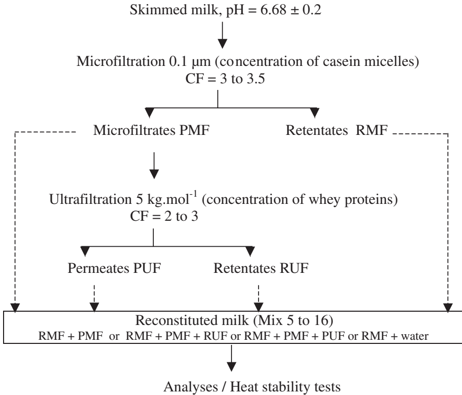
Figure 2. Schematic outline of the combined process used to prepare modified milk with either high micellar casein or high and low whey protein contents.
