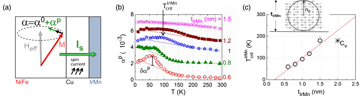
FIG. 3. (a) The spin pumping experiment. (b) Temperature ( T ) dependence of the IrMn spin pumping contribution to NiFe damping ( \alpha^P ). To facilitate reading, data have been shifted vertically. The enhanced spin pumping occurring during the IrMn magnetic phase transition is \delta\alpha^P . (c) Dependence of T_{crit}^{IrMn} on t_{IrMn} , where T_{crit}^{IrMn} is the critical temperature for the IrMn magnetic phase transition. Data fitting returns the spin-spin correlation length ( n_0 ). Adapted from Frangou et al. , 2016.
