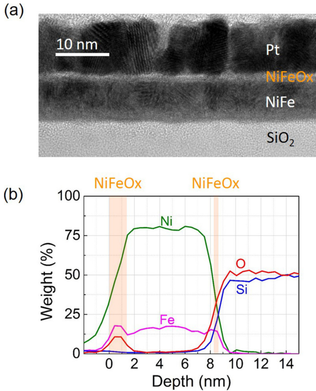
FIG. 1. (a) Transmission electron microscopy image (TEM) and (b) energy-dispersive x-ray spectroscopy (EDX) data for a \text{SiO}_2/\text{NiFe} sample. Samples were capped with Pt in preparation for the TEM experiment.
