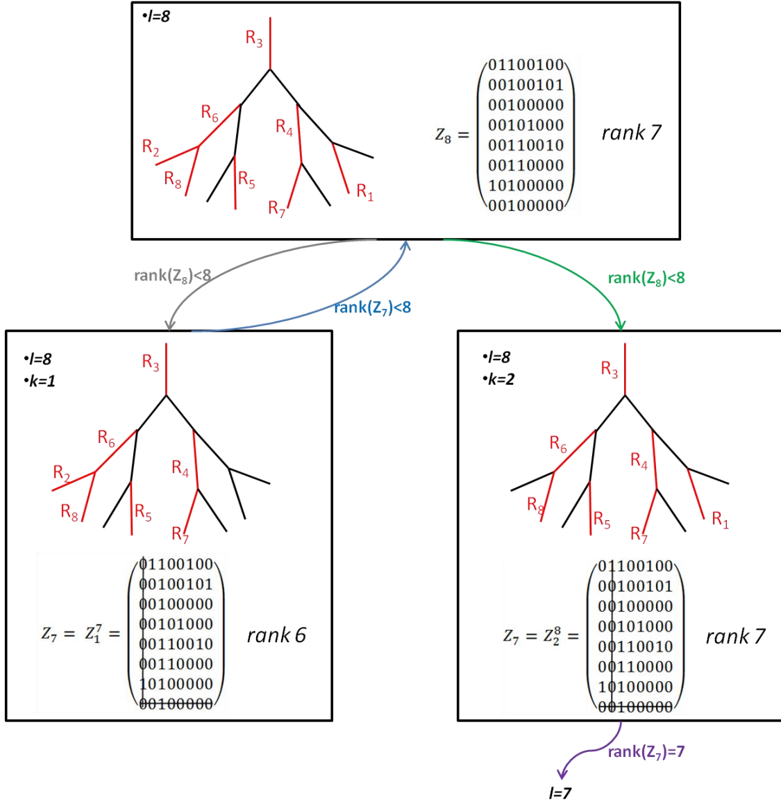
Figure 4: illustration of the resistance removal algorithm on an eight-exit tree. Branches in red are these with unknown resistance. Matrix Z_8 of the initial system is not invertible (top square). Following the process described in Figure 3, R_1 is first removed from the set of unknowns, a line and a column are removed from Z_8 leading to Z_7 (bottom left square); \text{rank}(Z_7) < \text{rank}(Z_8) so R_1 is set back among unknowns (top square) and R_2 is removed instead (bottom right square). Resulting reduced matrix Z_7 has now the same rank as Z_8 so the removal is confirmed. At the end of the process the tree contains several paths with R_{0,0} (= R_3) as only unknown, so a pressure along a path can be computed so as to solve the minimization problem (10), see Remark 2.
