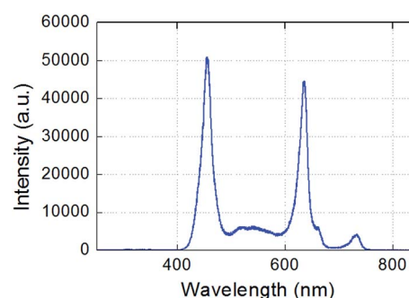
Fig. 2 Emission spectrum of the horticultural lamp.
