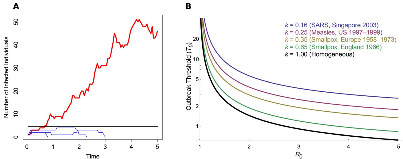
Figure 1. The outbreak threshold in homogeneous and heterogeneous populations. (A) A schematic of pathogen emergence. This graph shows the early stages of several strains of an epidemic, where R_0 = 1.25 . The black line denotes the outbreak threshold ( T_0 = 1/\text{Log}(R_0) = 4.48 ). Blue thin lines show cases in which the pathogen goes extinct and does not exceed the threshold; the red thick line shows an epidemic that exceeds the threshold and persists for a long period of time. Simulations were based on the Gillespie algorithm [22]. (B) Outbreak threshold in a homogeneous (black thick line) or in a heterogeneous population, for increasing R_0 . The threshold was calculated following the method described by Lloyd-Smith et al. [11] and is shown for different values of k , the dispersion parameter of the offspring distribution, as obtained from data on previous epidemics [11]. If the threshold lies below one, this means that around only one infected individual is needed to give a high outbreak probability. doi:10.1371/journal.ppat.1003277.g001
