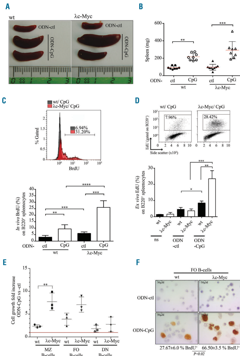
Figure 5. Effect of TLR9 stimulation on B cells from 4-5-week old \lambda c-Myc (pre-tumor stage) and wild-type (wt) mice. In vivo stimulation with control (ODN-ctl) or CpG containing (ODN-CpG) oligodeoxynucleotides: 10-fold 50 \mu g ODN intraperitoneal injection every two days. Representative spleen size (A) and scatter plot from spleen weight (B). B220 positive splenocyte proliferation after in vivo BrdU incorporation for about 24 hours (C): upper panel, overlay of representative BrdU labeling histograms gated on B220 positive cells from ODN-CpG injected \lambda c-Myc and wt mice; and lower panel, mean of in vivo BrdU percentage on B220 positive splenocytes. Data are shown as mean \pm standard deviation (n=6 mice in each experiment group). (D) Total splenocytes were ex vivo stimulated or not (ns) with control (ODN-ctl) or CpG containing motif (ODN-CpG) oligodeoxynucleotides. Proliferation at day 4 was assessed by EdU incorporation and labeling of B220 positive splenocytes. Upper panel: representative biparametric EdU side scatter cytograms gated on B220 positive cells. Percentages of EdU+ and B220+ cells are indicated in each graph. Lower panel: mean percentages of EdU+ and B220+ cells. Data are shown as mean \pm standard deviation (n=4 mice in each experiment group). (E) Cell growth of marginal zone (MZ), follicular (FO) and double negative (DN) spleen B cells sorted from wt and \lambda c-Myc mice. Cells were counted by Trypan blue staining exclusion after 4 days stimulation. Red line indicates no cell growth fold increase in ODN-CpG condition versus ODN-ctl condition (value = 1). Data are shown as mean \pm standard deviation (n=3 mice in each experiment group). (F) BrdU labeling of sorted FO B cells from wt (left panels) and \lambda c-Myc mice (right panels) treated (CpG, lower panels) or not (ctl, upper panels) with CpG oligonucleotides for 4 days. BrdU incorporation was performed 4 hours before cells were cytoцентрифугed. No BrdU incorporation was detectable in ctl conditions (upper panels). Mean and standard deviation of percentages of BrdU positive CpG treated cells are indicated (n=3 mice in each experiment group). Statistical significance was determined by Student's t -test (*** P <0.0001; ** P <0.001; * P <0.01; * P <0.05). EdU: 5-ethynyl-2'-deoxyuridine; BrdU: 5-bromo-2'-deoxyuridine.
