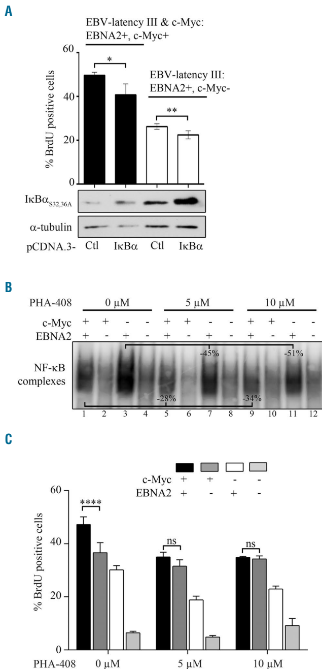
Figure 3. Activation of NF- \kappa B in P493.6 cells after induction of c-Myc on EBV-latency III. P493.6 cells were treated or not with estradiol 1 \mu M (EBNA2- or EBNA2+) and/or with tetracycline at 100 ng/mL (c-Myc+ or c-Myc-) for 48 hours. (A) Percentage of BrdU positive cells after transient transfection with the pCDNA.3 empty vector (Ctl) or expressing the super-repressor I \kappa B \alpha S32,36A for 48 hours (upper panel). Representative analysis of I \kappa B \alpha S32,36A , and \alpha -tubulin expression by Western blot (lower panel). (B and C) Effect of the IKK2 inhibitor PHA-408 (5 \mu M and 10 \mu M) for 48 hours on NF- \kappa B. Representative DNA binding by EMSA (panel B) and BrdU incorporation (panel C). In the histograms, data are shown as the mean \pm standard deviation (at least 3 independent experiments). Statistical significance was determined by Student's t -test (**** P <0.001; ** P <0.01; * P <0.05). ns: not significant; BrdU: 5-bromo-2'-deoxyuridine; EBNA2: Epstein-Barr virus nuclear antigen 2; EBV: Epstein-Barr virus; Ctl: control; NF- \kappa B: nuclear factor- \kappa B.
