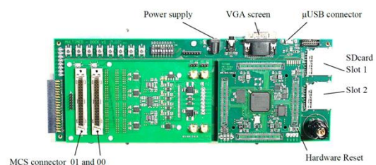
Figure 1: Picture of the neuromorphic board used for this study.
