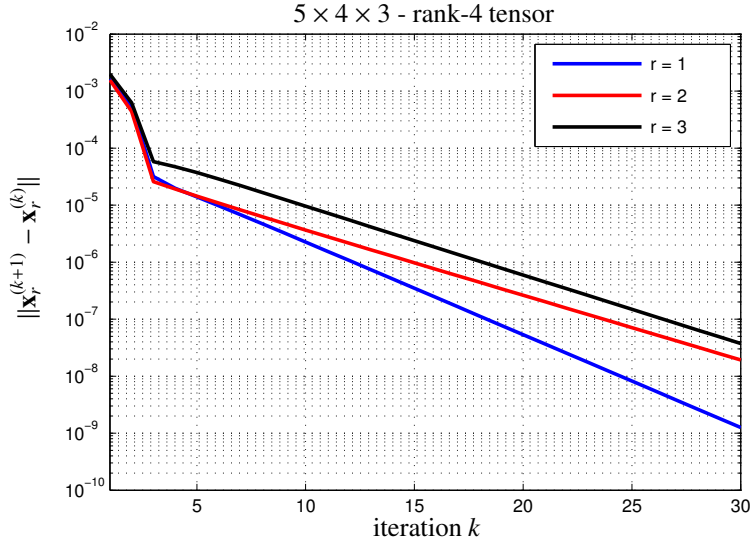
Figure 2: Convergence of the iterates in CAPD algorithm for a single rank-4 tensor.
