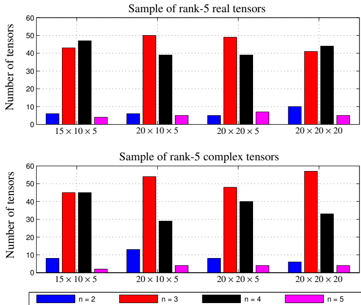
Figure 3: Tensors for which n column factors are correctly extracted with the all-at-once algorithm.
