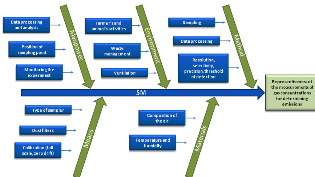
Figure IX. Application of an Ishikawa diagram for measuring gas concentrations in ambient air in a livestock building
