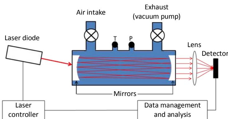
Figure M12.2. Off-Axis Integrated Cavity Output Spectroscopy
