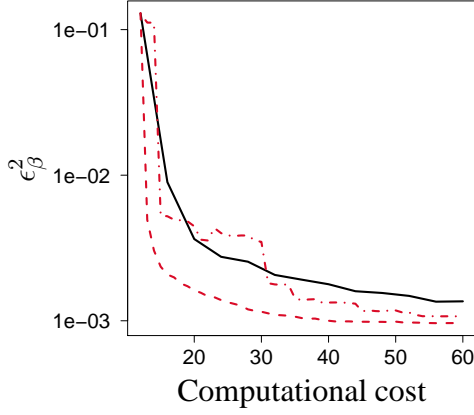
(a) Analytic example : Calibration
