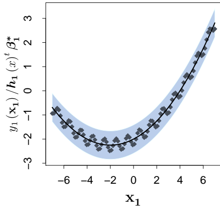
(a) Phenomenon 1 : computer model (initial process)
