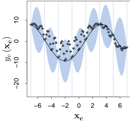
(a) 8 observations : Black-box
