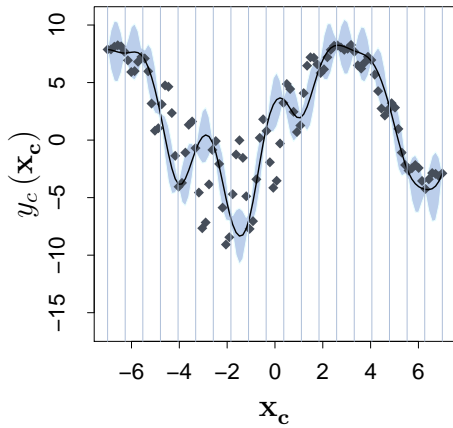
(c) 20 observations : Black-box
