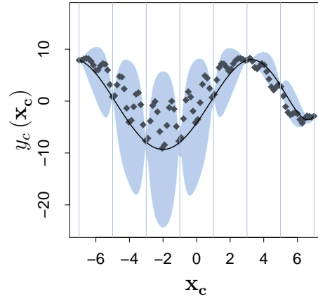
(b) 8 observations : A posteriori linearized
