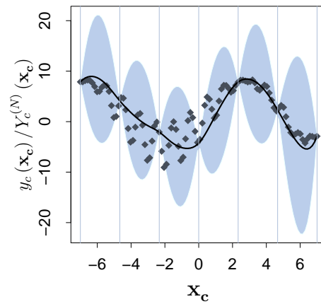
(f) Nested phenomenon : estimator (conditional process)
