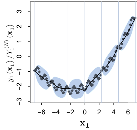
(b) Phenomenon 1 : estimator (conditional process)
