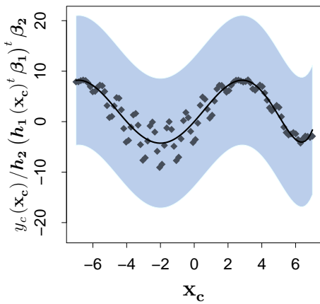
(e) Nested phenomenon : computer model (initial process)
