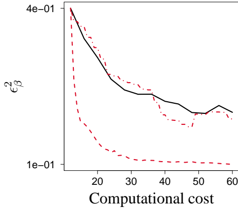
(c) Hydrodynamic example : Calibration
