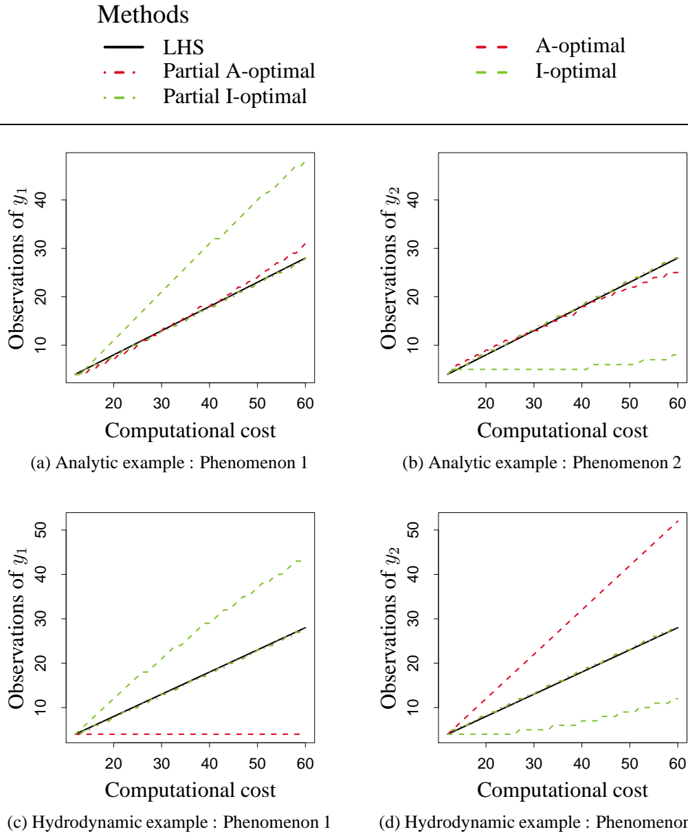
Figure 8: The figures represent the number of observations of the phenomena 1 and 2 for the different studied designs.
