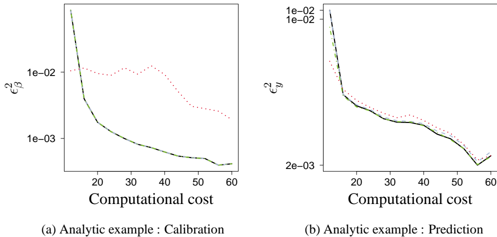
Figure 4: The figures represent the performance of calibration and prediction for the previously presented approaches (parallel with Monte-Carlo, parallel with analytical formula, a priori and a posteriori linearized). The observations are drawn according to chained Latin Hypercube designs (LHS) of increasing size. The observations' choice is repeated 50 times. The covariance functions of \epsilon_1 and \epsilon_2 are Gaussian.
