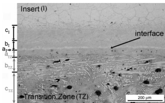
2 Optical micrograph of region around insert/transition zone interface (etched with Vilella)
