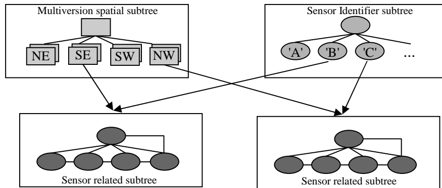
Figure 6: PasTree structure
