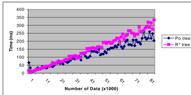
Figure 5: influence of the number of data on spatial windows / temporal interval queries (last 10% of the entered data)
