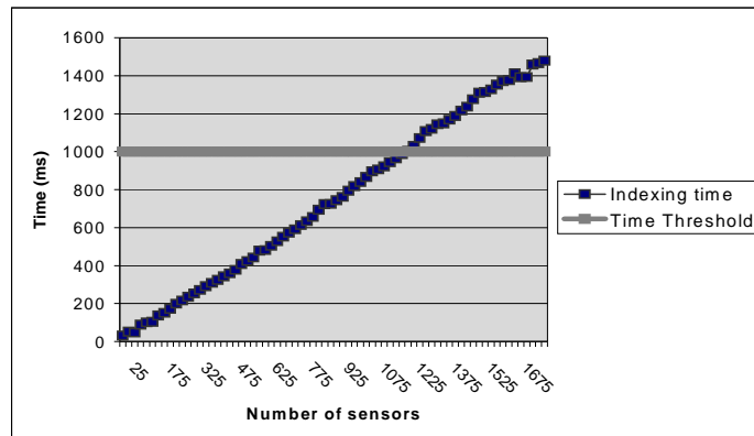
Figure 3: influence of the number of fixed sensors on the construction time of the PoTree
