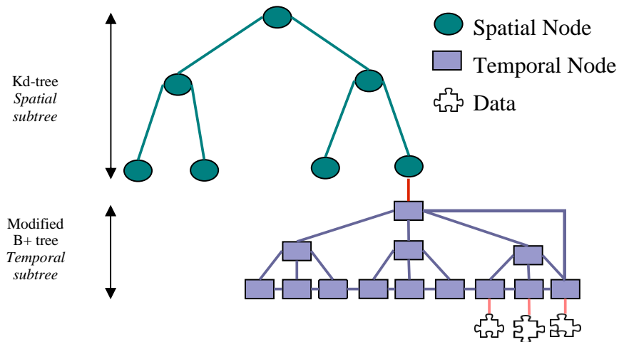
Figure 2: PoTree structure
