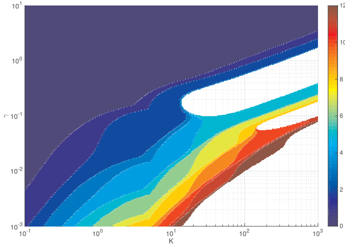
Fig. 1. Stability region in the plan (K, \gamma) , obtained using Theorem 1 for N = 0, \dots, 12 .
