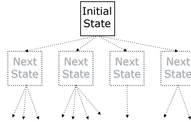
Nondeterministic Choice
