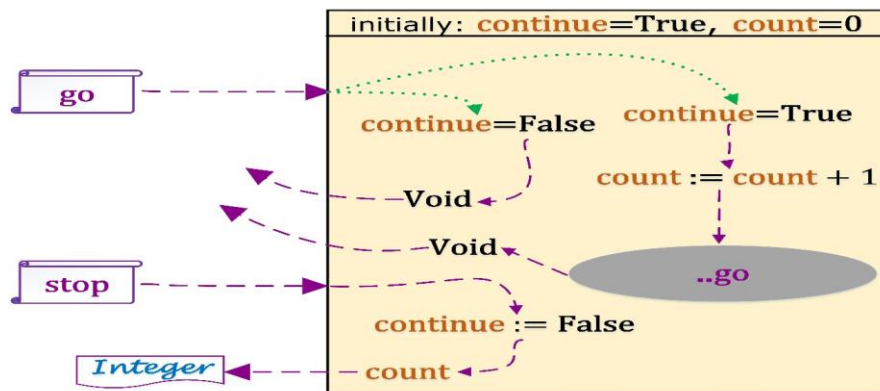
Actor with message passing indeterminacy
