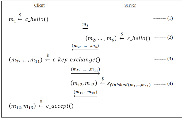
Fig. 1. TLS 1.2 negotiation (Ephemeral Diffie-Hellman)
