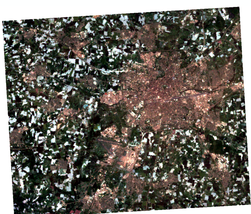
Image Landsat 5 (RVB)
