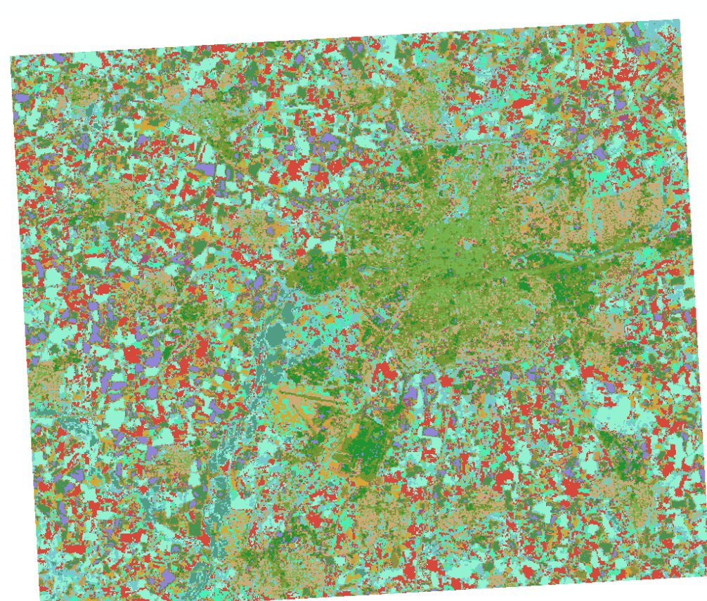
Classification (15 classes)
