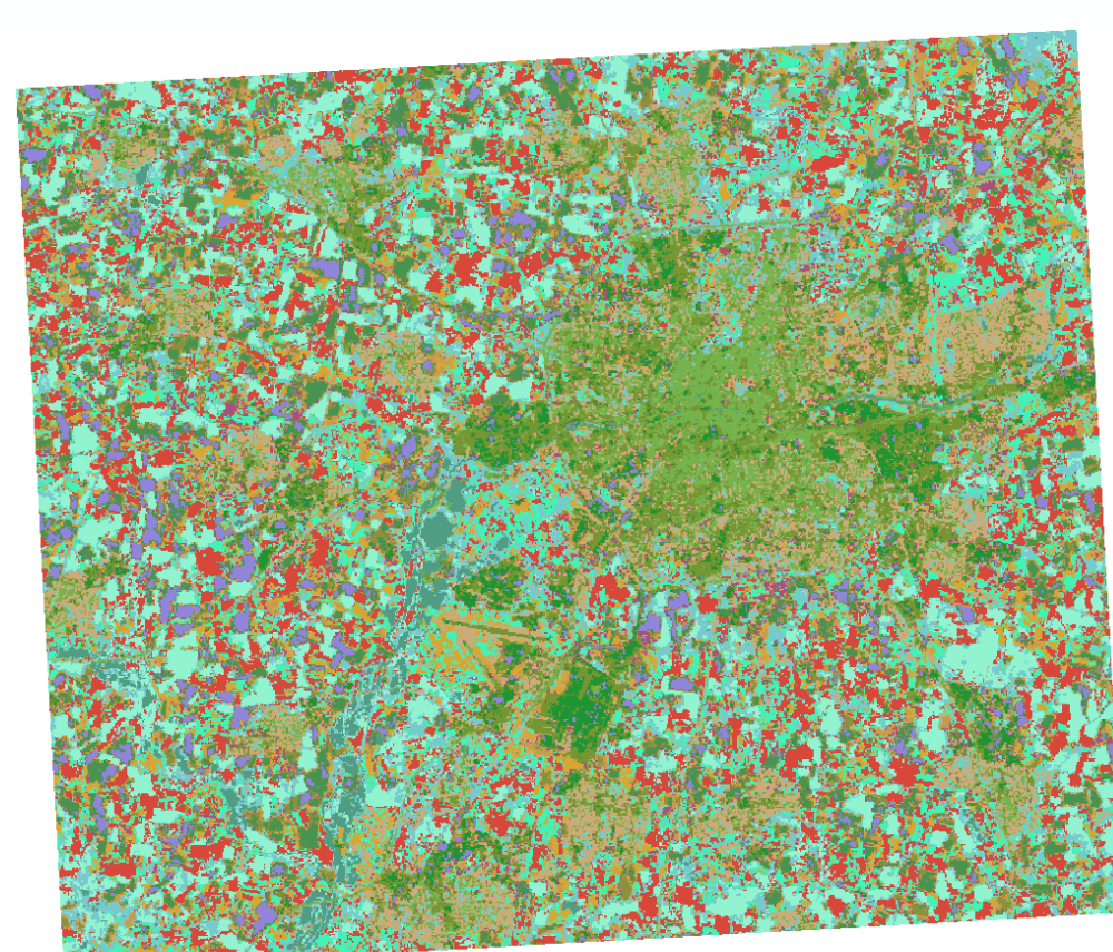
Classification (15 classes)
