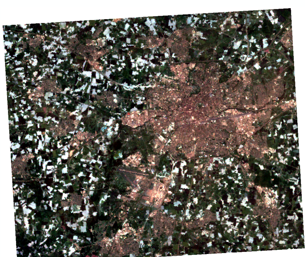
Image Landsat 5 (RVB)
