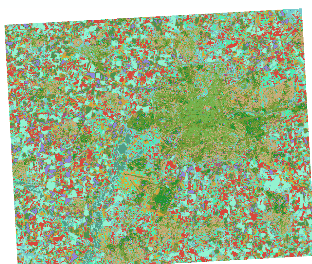
Classification (15 classes)
