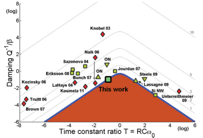
FIG. 9. (Color online) Normalized dissipation 1/Q\beta as a function of the time constant ratio T = \omega_0 RC for various reported experiments (logarithmic axes). The continuous line is the universal electrostatic damping \Gamma_{\text{es}}/(\beta\omega_0) from Eq. (4). It sets a theoretical lower limitation (lower region) for the dissipation. The linear increasing and decreasing slopes correspond, respectively, to the asymptotic regime calculated in Eqs. (6) and (8). The experimental data are plotted using quality factor, capacitance ratio \beta , and time ratio T for bottom-up (squares) (Table III) and top-down devices (diamonds) (Table IV). Lassigne 09 ( \Delta ) and Steele 09 ( \nabla ) data correspond to the Coulomb blockade regime. The ON associated triangles correspond to the Coulomb peaks when the resonator is in its conductive regime. The vertical distances from the electrostatic damping lower limit give the additional source of dissipation.
