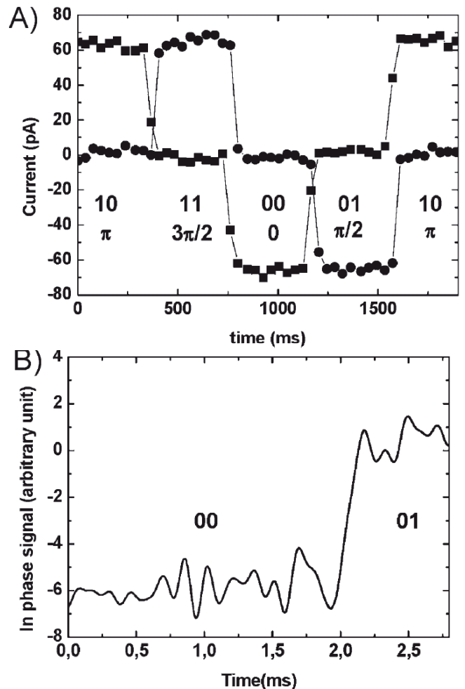
FIG. 8: a) Schematic Digital demodulation (■ in phase and ● out of phase component) for \omega_\Delta/2\pi = 200\text{kHz} , \omega_L/2\pi = 616.3\text{Hz} , \omega_c/2\pi = 112.8\text{MHz} , V_g = -9.5\text{V} , A = 20\text{mV} and a time constant of 10 ms. B) High speed digital demodulation for \omega_\Delta/2\pi = 750\text{kHz} , \omega_L/2\pi = 7243\text{Hz} , \omega_c/2\pi = 156.98\text{MHz} , V_g = 9\text{V} , A = 20\text{mV} and a time constant of 30 \mu s.
