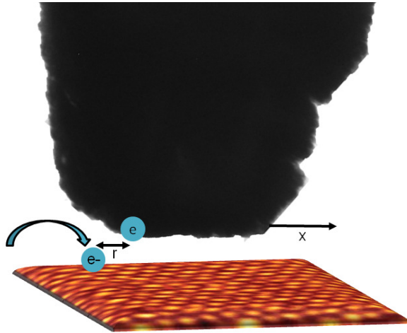
Figure 5: Model use to evaluate the influence on the probe resonance of fluctuating charges on surface. The relative frequency variation can be estimated from the spring constant variation. The effect of a single electron on surface is consistent with the measured frequency fluctuation (see text).
