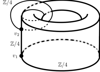
(B) Orbit space of the displayed fundamental domain for \Gamma_0(\sqrt{-2}) , with the cusp having become a 2-torus in the Borel–Serre compactification. The 2-torsion subcomplex is given by the edges labeled by \mathbb{Z}/4 , and their vertices.
