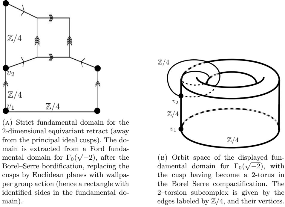
FIGURE 5. Fundamental domain for \Gamma_0(\sqrt{-2}) \subset \mathrm{SL}_2(\mathbb{Z}[\sqrt{-2}])
