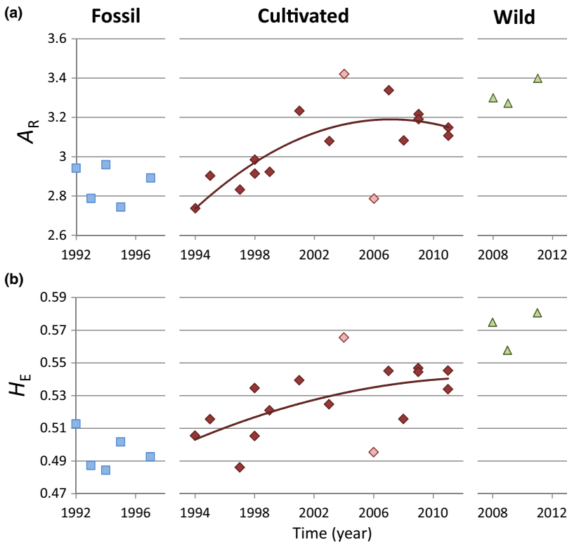
Fig. 5 Temporal evolution of neutral genetic diversity: (a) allelic richness ( A_R ); (b) gene diversity ( H_E ). Populations are sorted according to the three genetic groups identified by TESS analysis: the fossil, cultivated and wild populations, respectively, in blue, red and green. The two samples with the smallest sample size (cultivated population) are figured by faded diamond dots. [Colour figure can be viewed at wileyonlinelibrary.com ]
