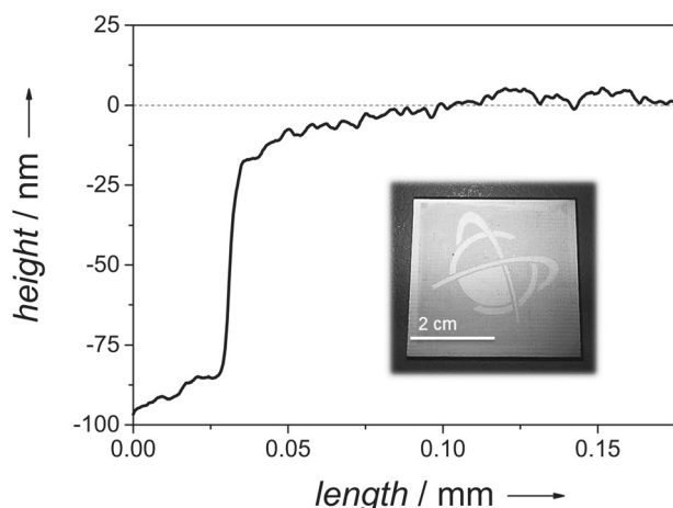
Figure 1. Height profile of a film of pNonOx 80 -stat-pDc=Ox 20 after illumination and development. The copoly(2-oxazoline) had been spincoated on a gold-coated FR4 substrate and been illuminated through a mask.
