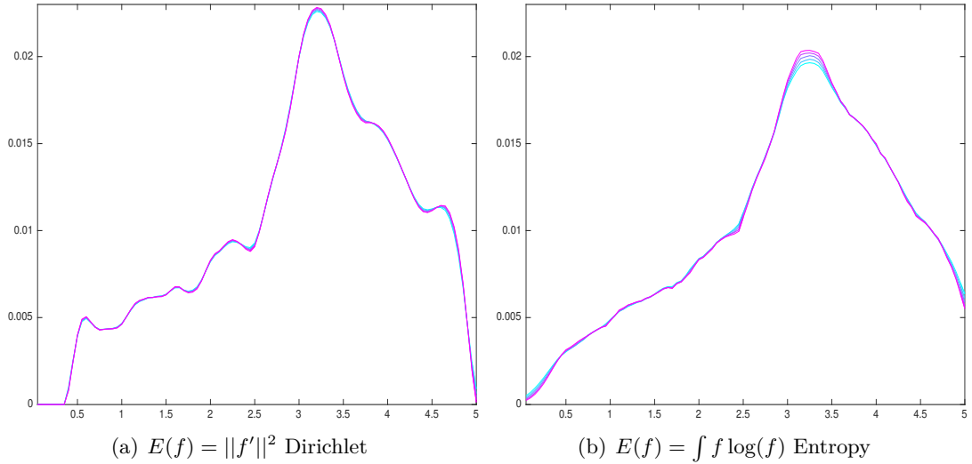
Figure 6: Neural spike trains data. (a) Pdf of the regularized empirical Wasserstein barycenter with a Dirichlet regularization for 6 \leq \gamma \leq 10 . (b) Pdf of the regularized empirical Wasserstein barycenter with negative entropy regularization and 0.08 \leq \gamma \leq 0.12
