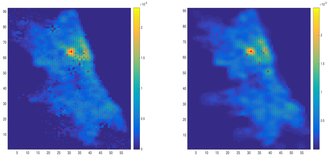
(a) Our approach: pdf of regularized Wasserstein barycenter with unregularized transport cost. (b) The approach in [CP16]: regularized Wasserstein barycenter with regularized transport cost and Sinkhorn's algorithm.
